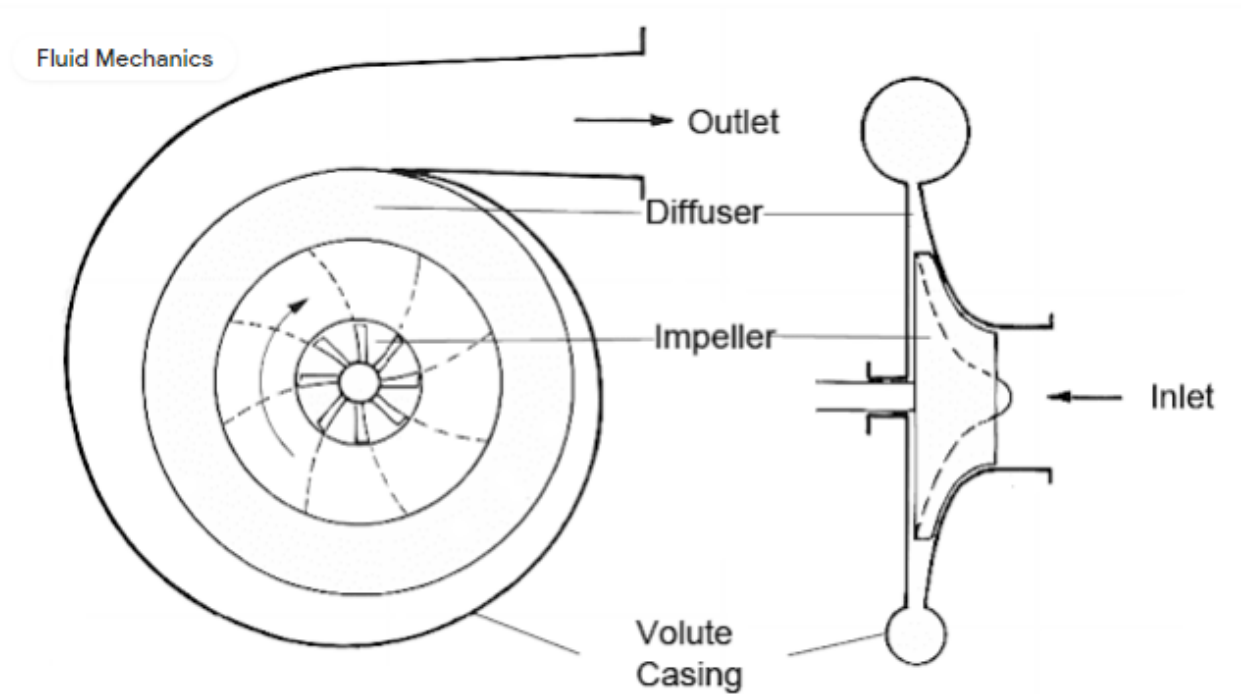
Centrifugal compressor schematic diagram
