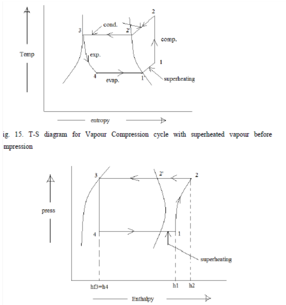
Fig. 16. P-h diagram for Vapour Compression cycle with superheated vapour before compression In this cycle, the evaporation starts at state 4 and continues up to the point 1.
